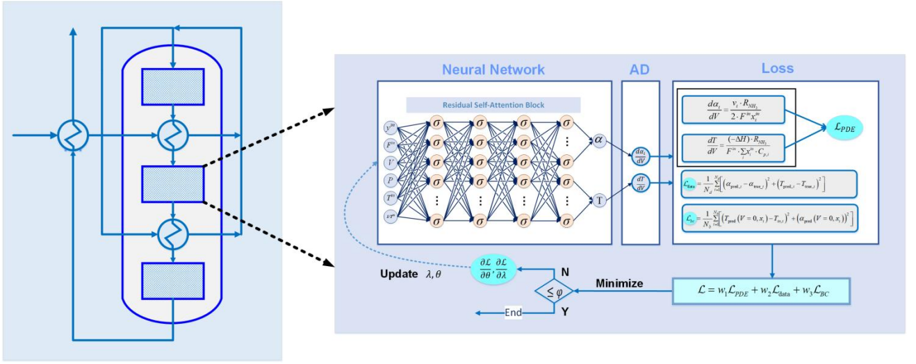
Fig. 1. Architecture and training framework of the residual-attention PINN, including the reactor physics constraints, network structure, and composite loss function.
