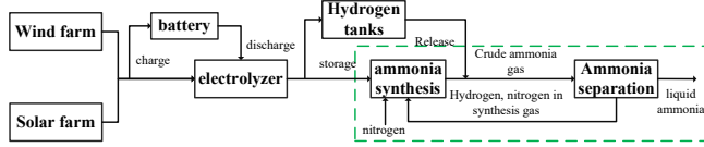
Fig. 1. Structure of the ammonia synthesis system under green hydrogen fluctuation
