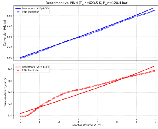
Fig. 3. Predicted axial profiles of N_2 conversion (top) and outlet temperature (bottom) from the PINN surrogate compared with ODE reference solutions at T_{in} = 623.5\text{ K} , P = 120.4\text{ bar} .
