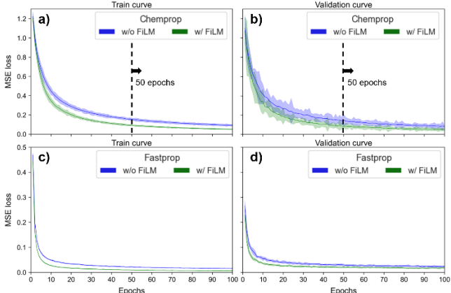
Figure 3. Training and validation curve for data-driven models with and without FiLM
