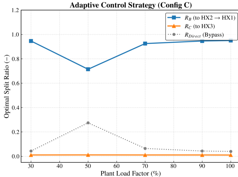
Fig. 10. Optimal split ratios for Config C as a function of plant load, obtained by surrogate-based optimization. R_B : flow fraction through inter-bed exchangers HX_1/HX_2 ; R_C : flow fraction through feed preheater HX_3 ; R_{direct} : direct bypass fraction.
