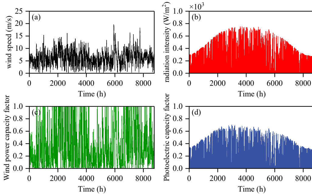
Fig. 2. Local annual meteorological data and corresponding wind and solar capacity factors: (a) wind speed data; (b) solar irradiance data; (c) wind power capacity factor; (d) solar power capacity factor.
