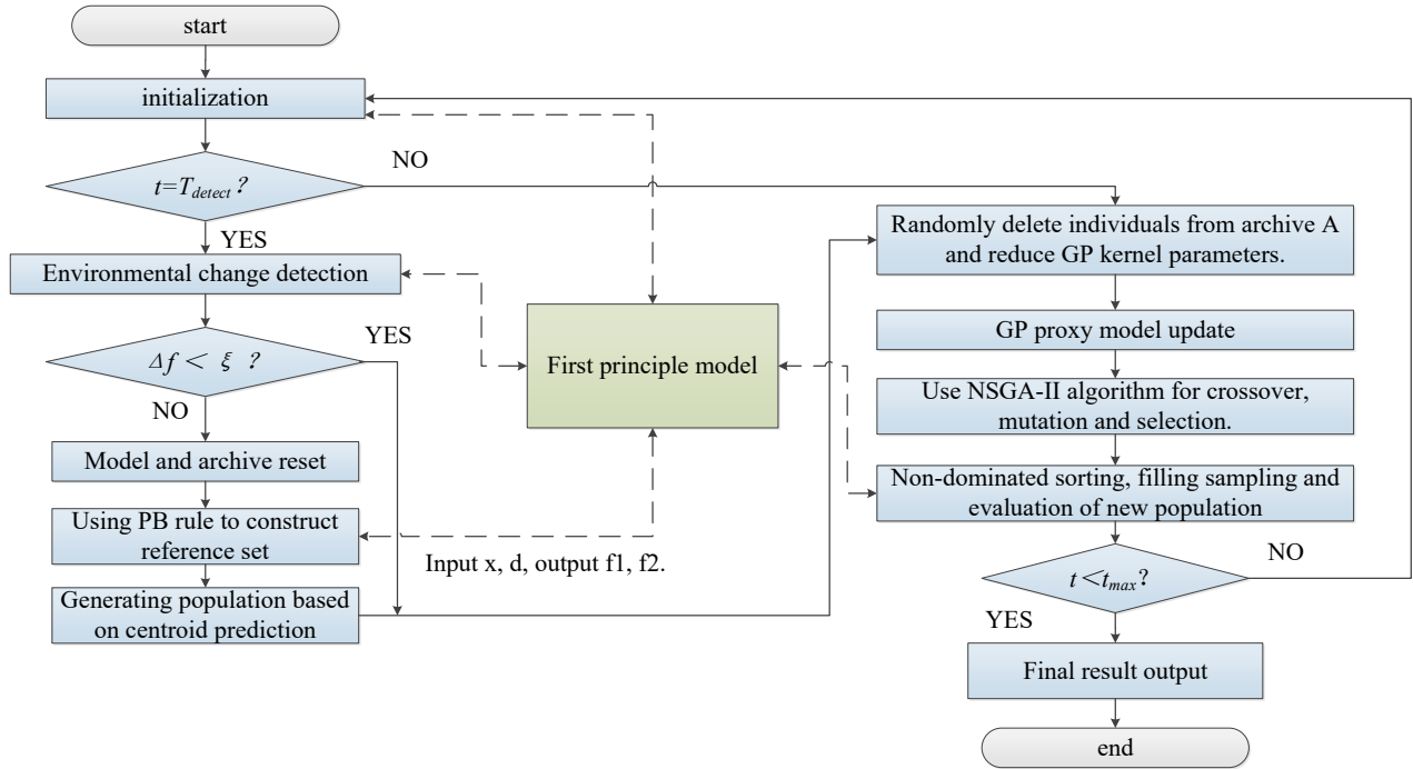
Fig. 3. Flowchart of the DAPB-NSGAll algorithm
