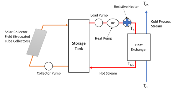
Figure 1. Schematic of the solar thermal system.
